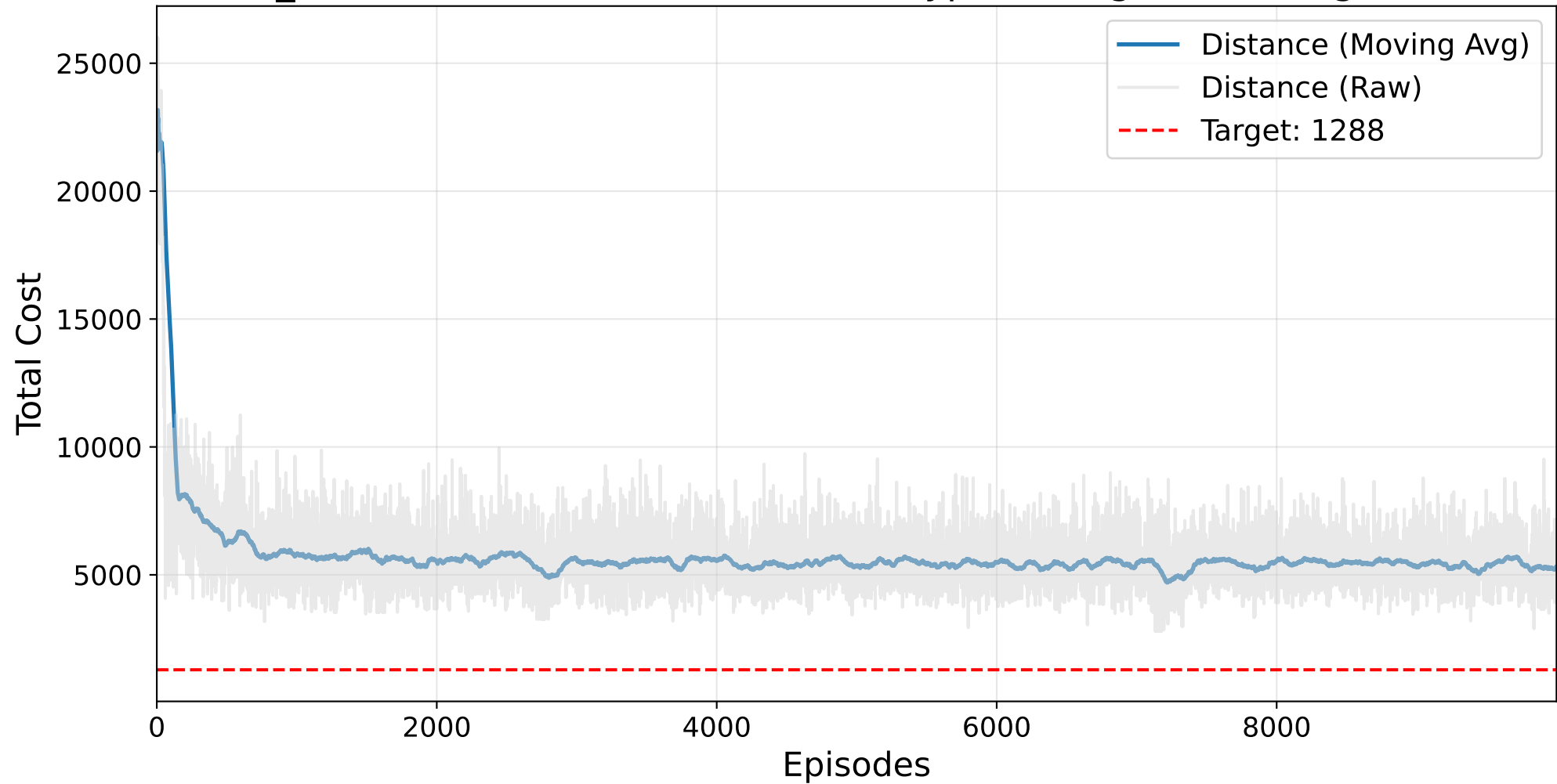
Final NO_BAYESIAN Masked AutoRL-SOP (HyperTuningSK) Training - ESC47.sop
